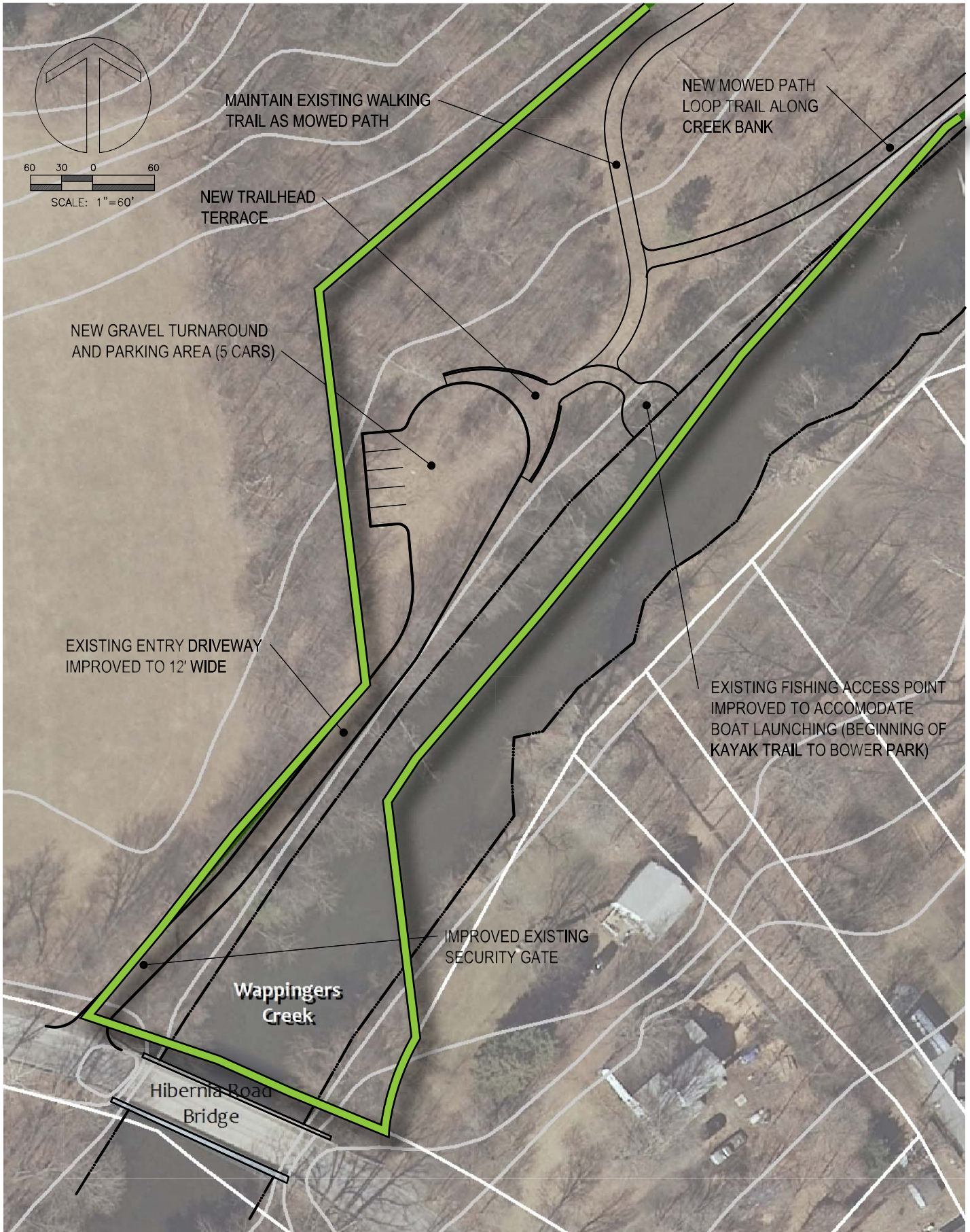
Figure 4-7 Hibernia Road Parcel Concept Plan
